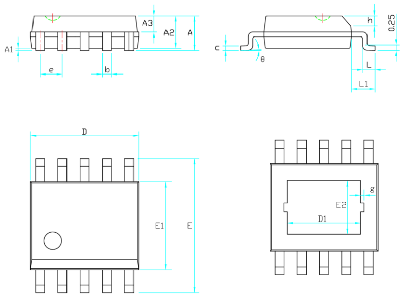
ESSOP10-8R(95*130) Package Outline Dimensions units:mm
