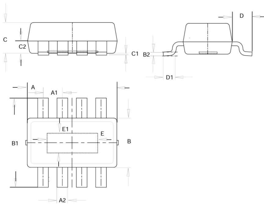
ESOT23-8L PACKAGE OUTLINE DIMENSIONS
