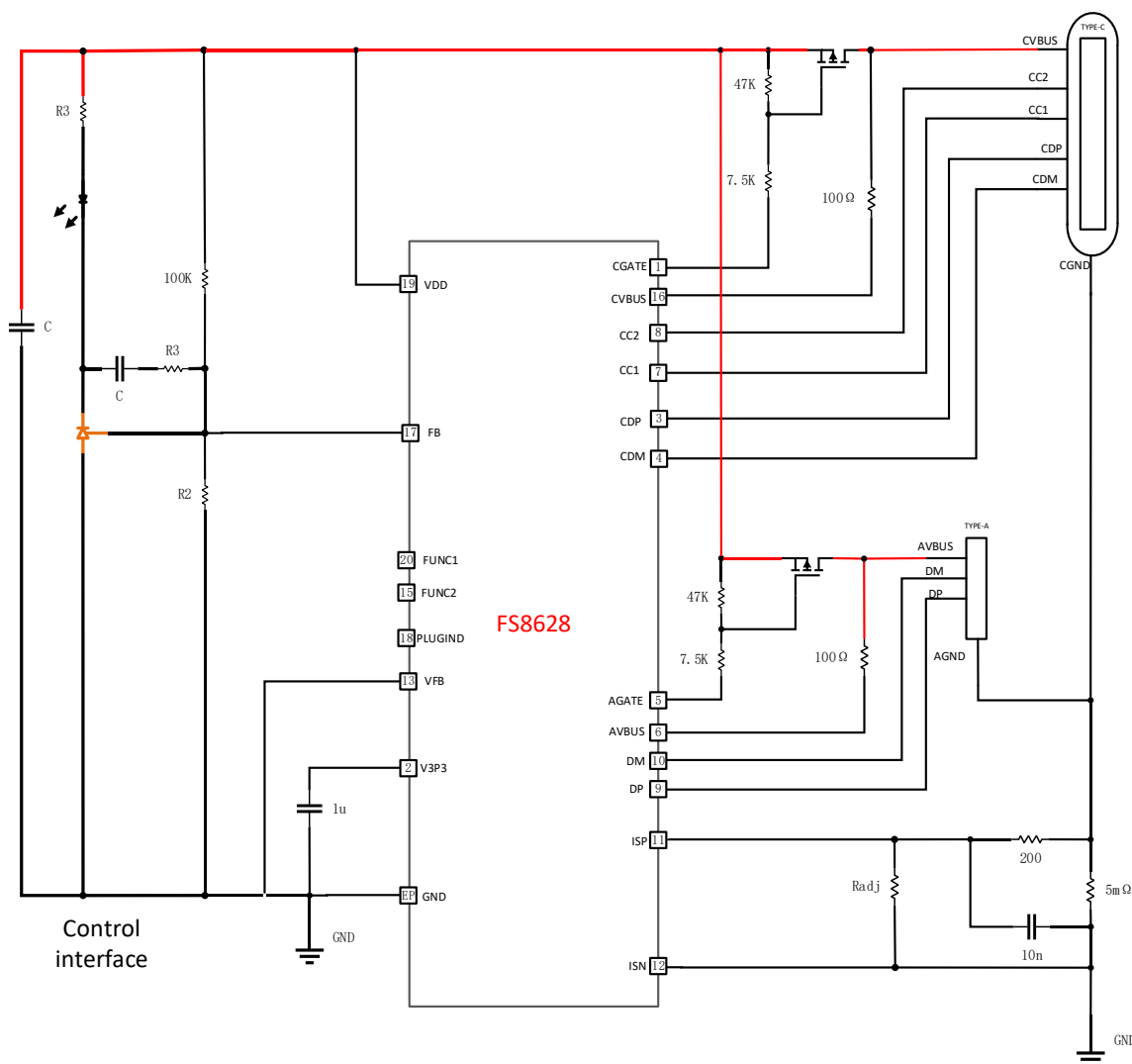
Figure 2. Application diagram of FS8628L
