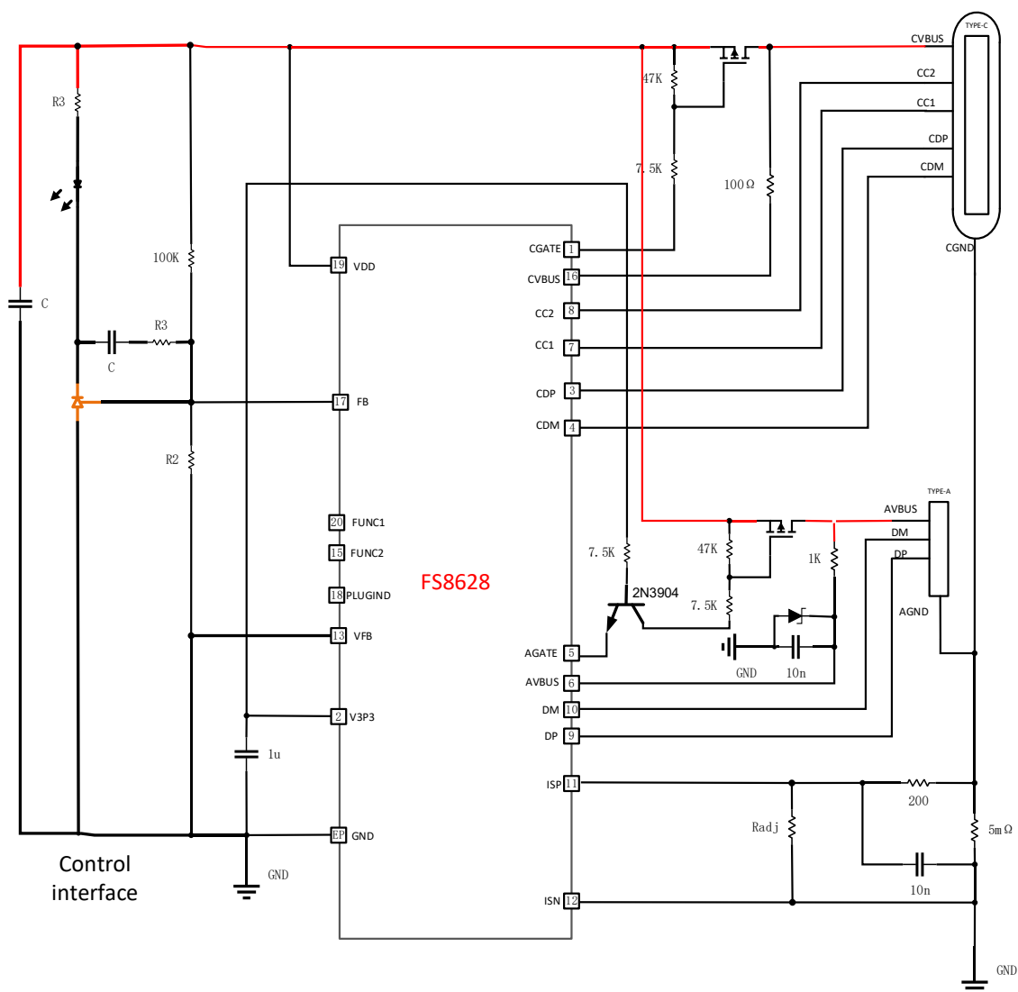
Figure 3. Application diagram of FS8628H
