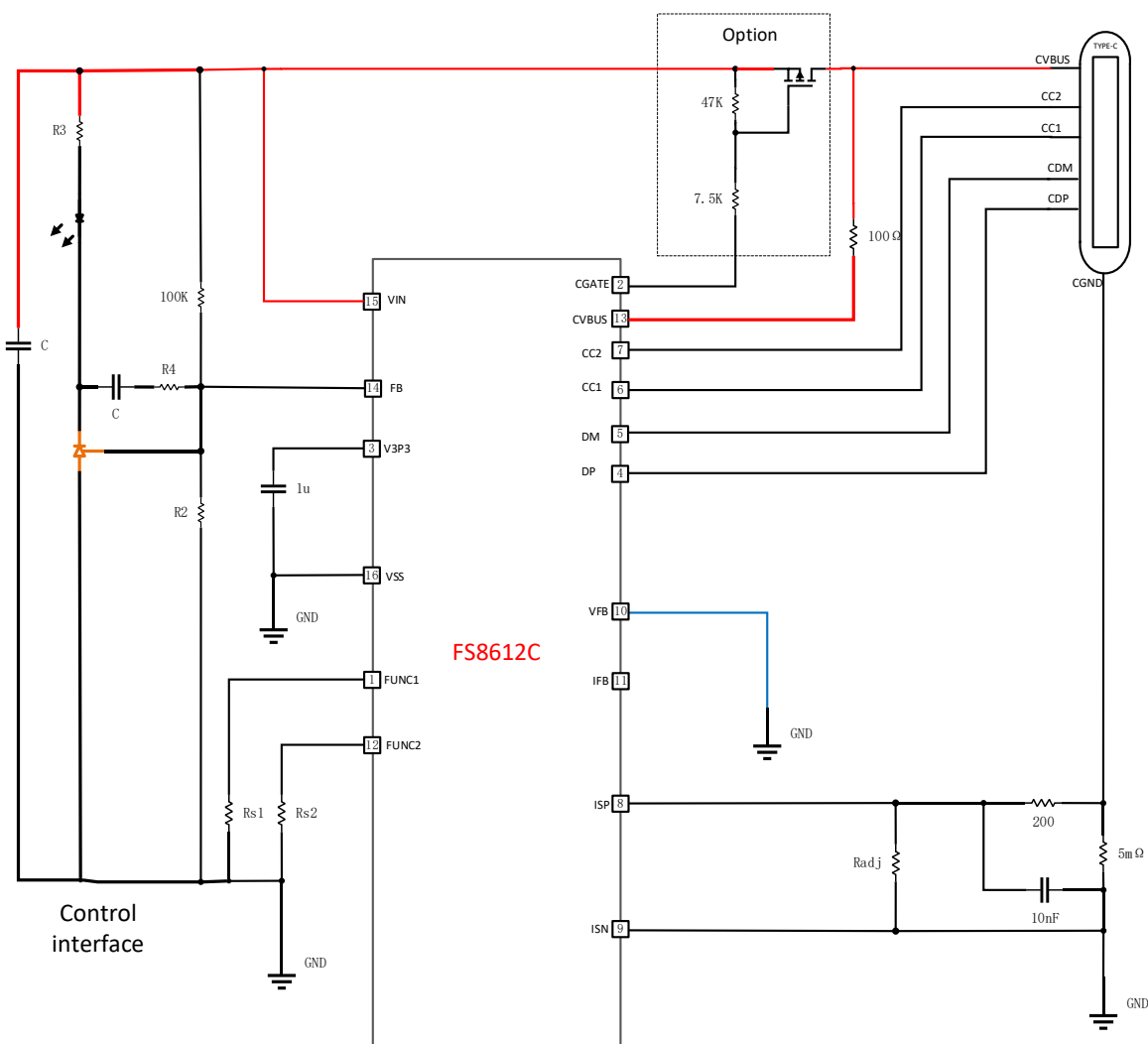
Figure 3. Application diagram of FB
