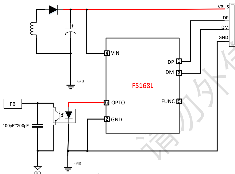
Figure 2. Application diagram
