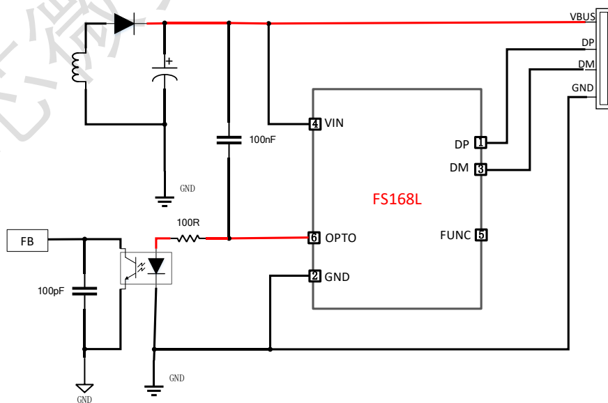
Figure 3. Application diagram
