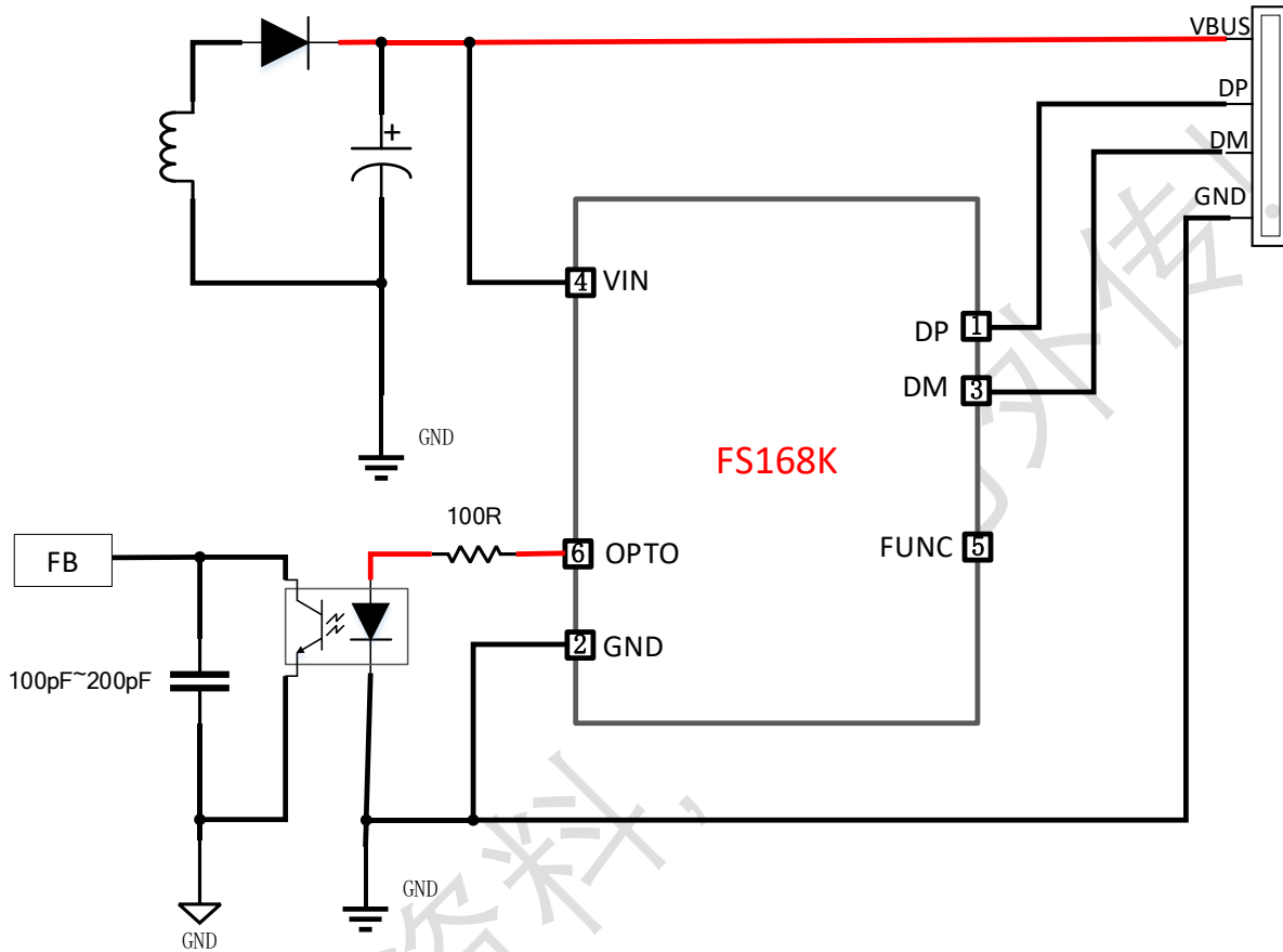
Figure 2. Application diagram
