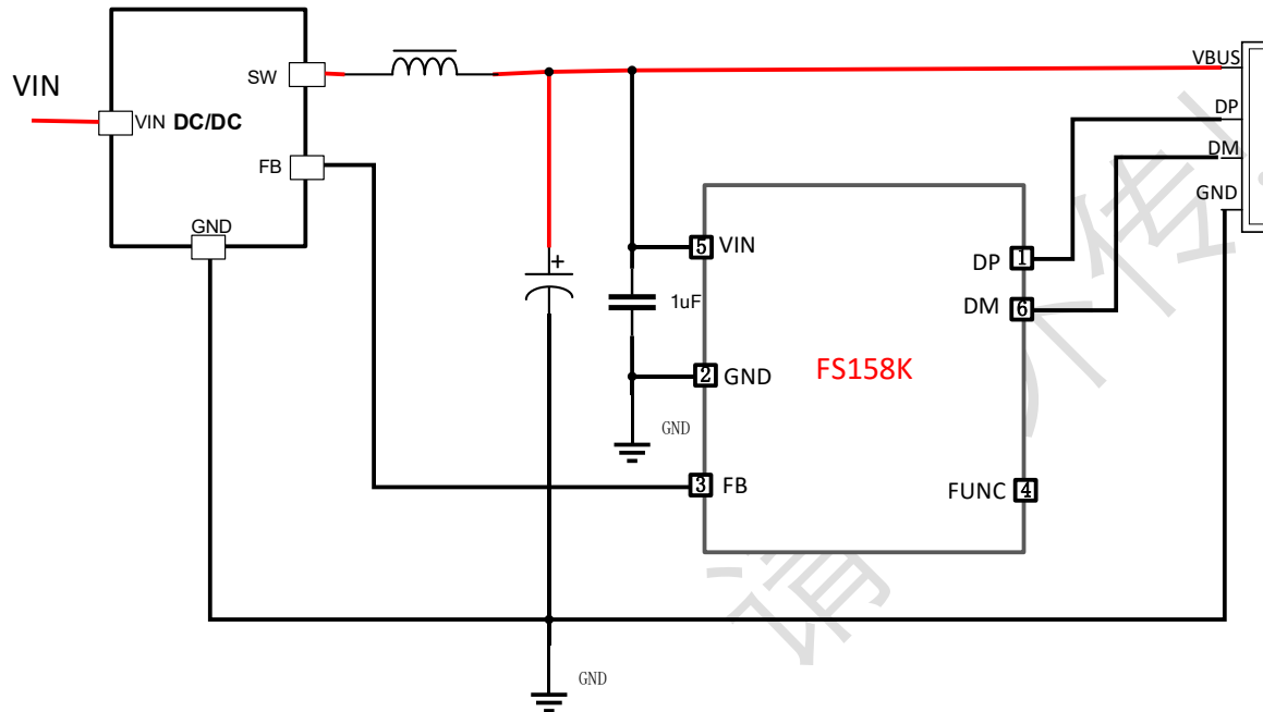
Figure 2. Application diagram
