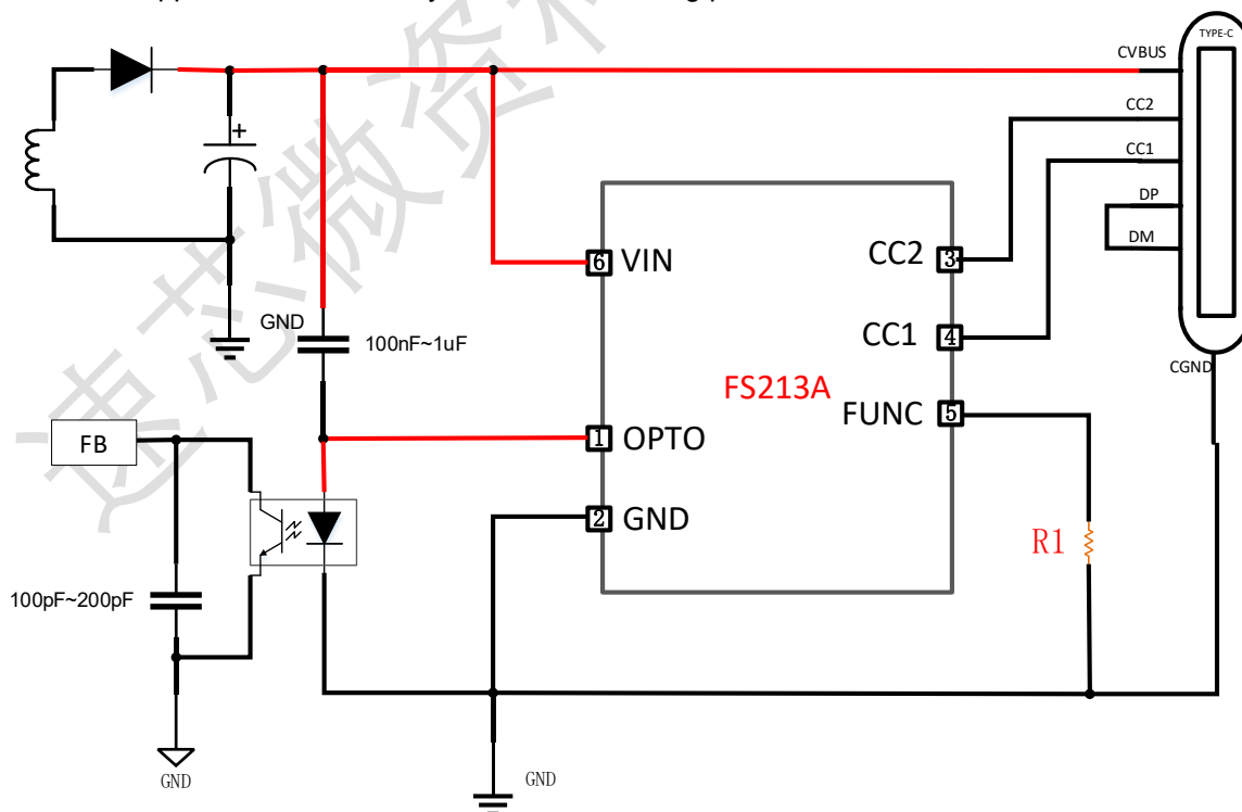
Figure 3. FS213A simulation MOS application diagram
