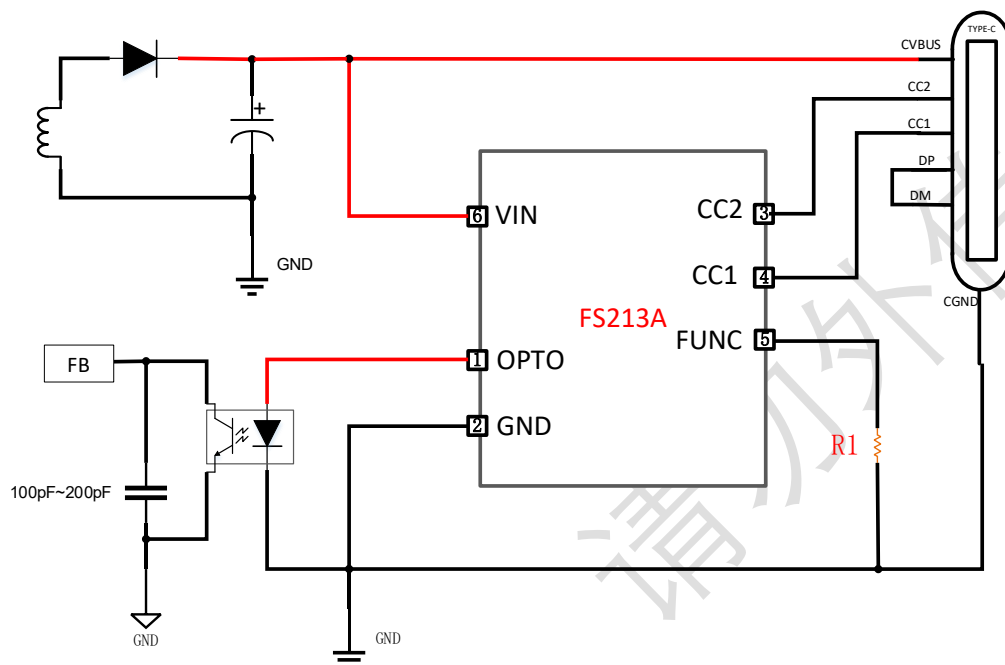
Figure 2. Application diagram
