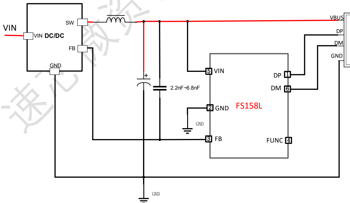
Figure 3. Application diagram
