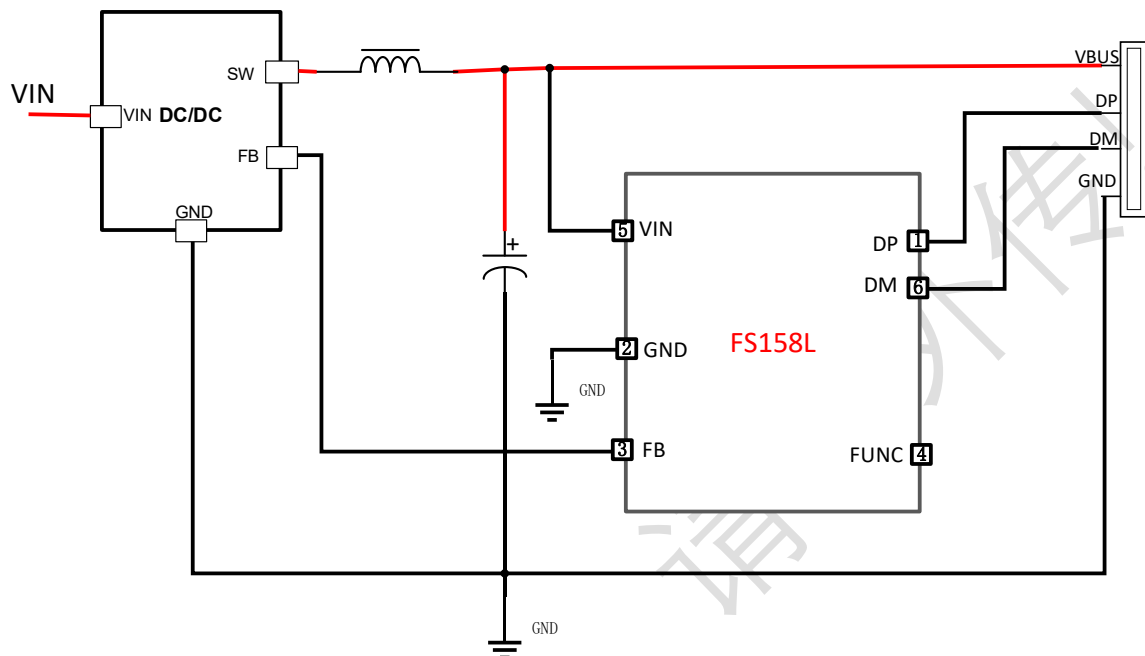
Figure 2. Application diagram
