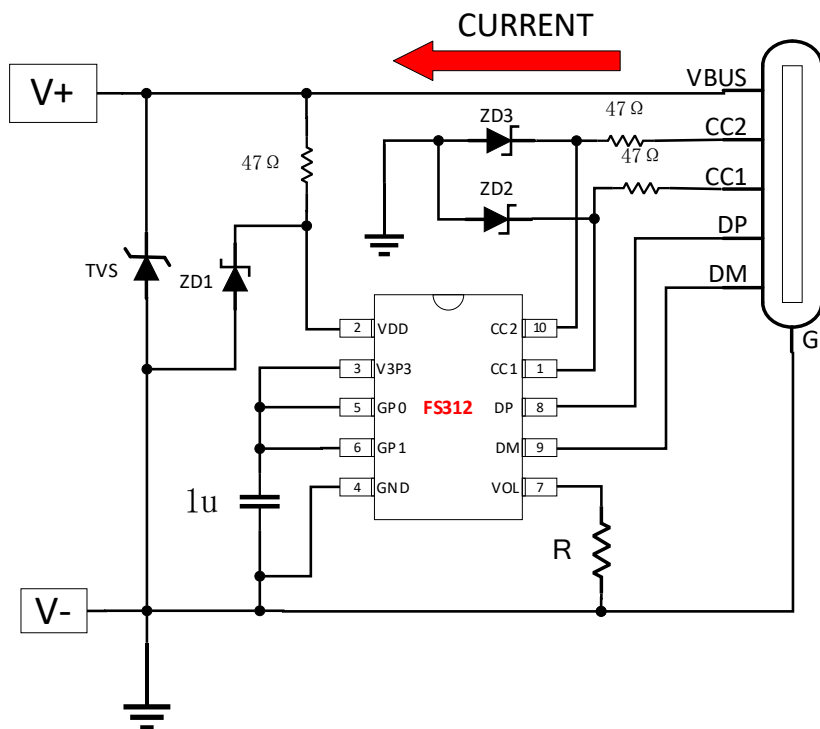
Figure 3. Application diagram
