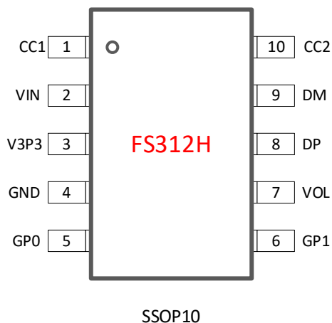
Figure 1. Pin Definition
