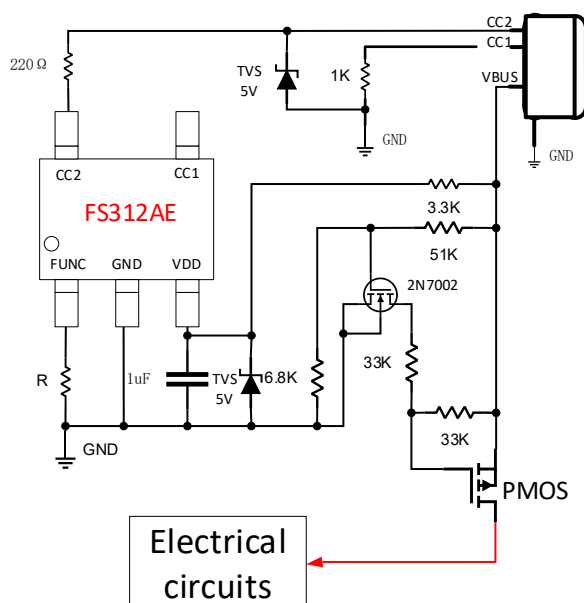
Figure 5. Application diagram
