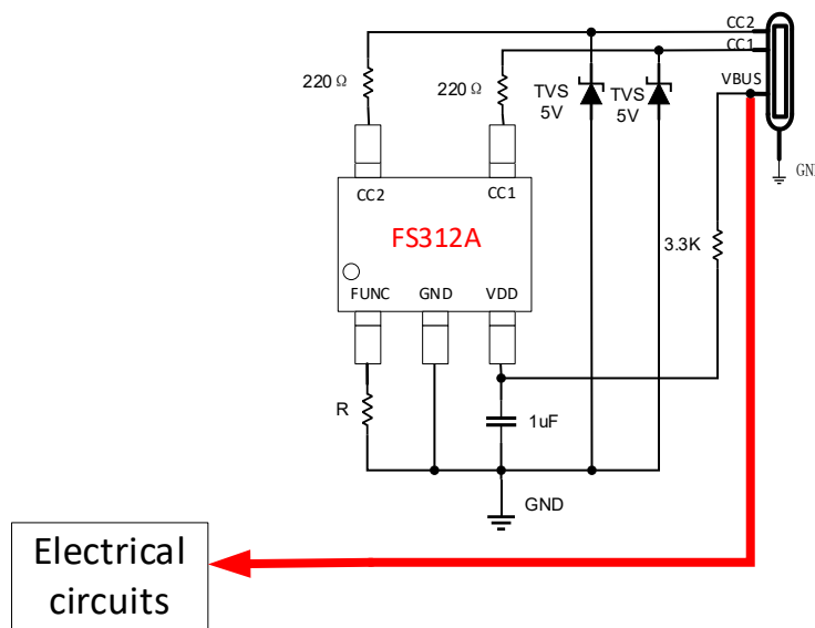
Figure 2. Application diagram
