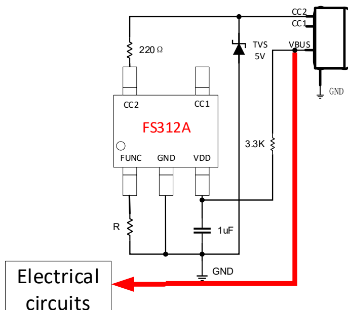
Figure 3. Application diagram
