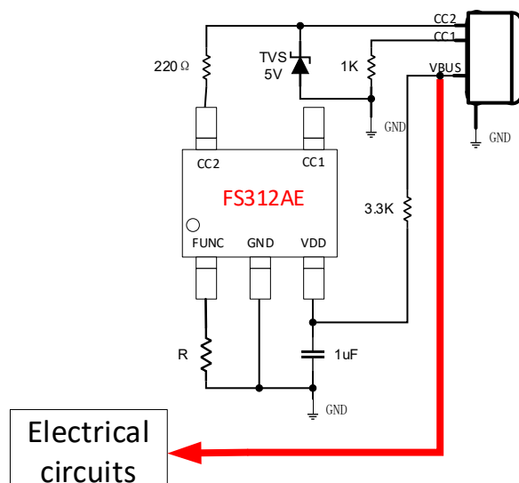
Figure 4. Application diagram
