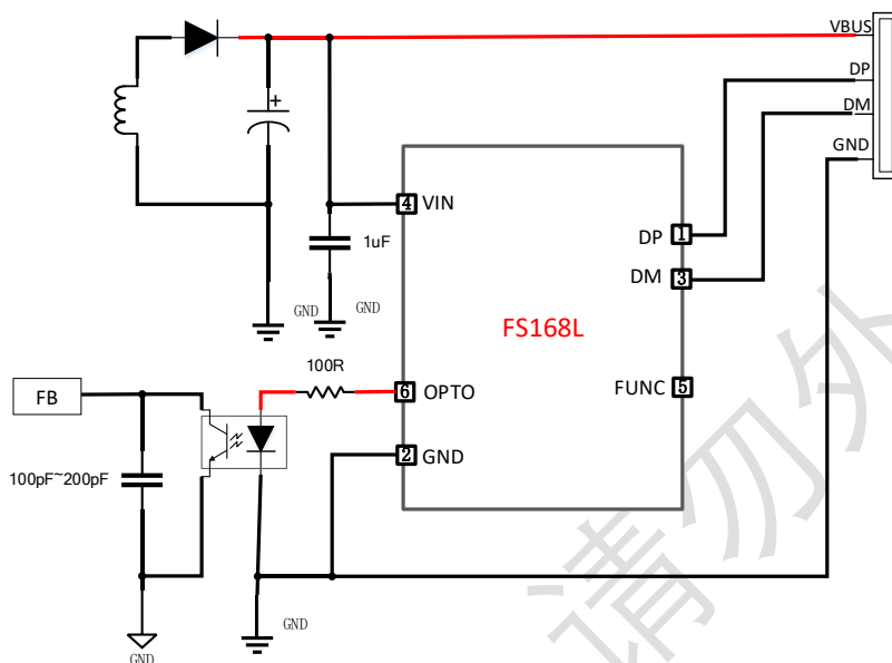
Figure 2. Application diagram
