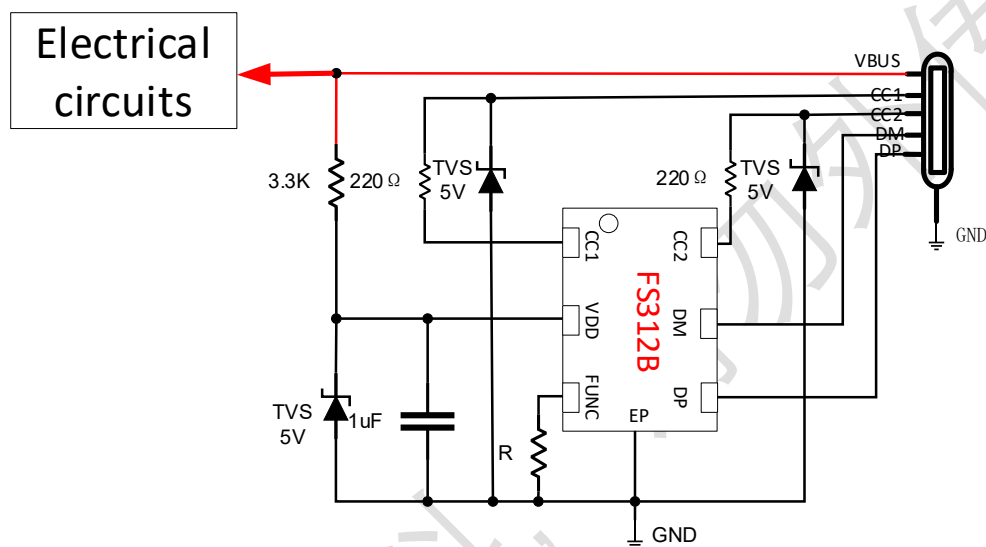
Figure 2. Application diagram
