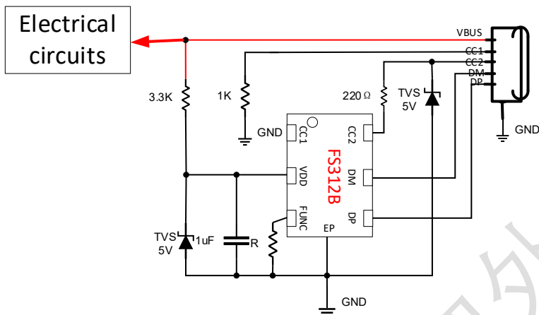
Figure 4. Application diagram
