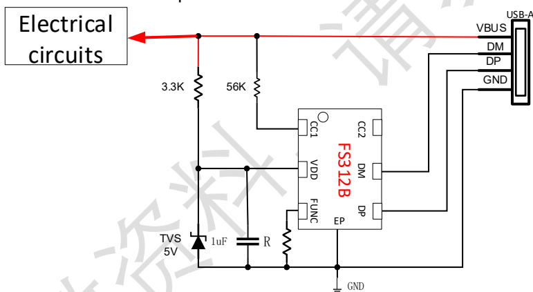
Figure 5. Application diagram
