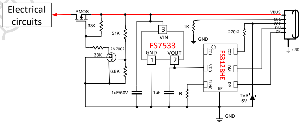
Figure 6. Application diagram
