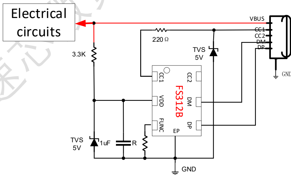
Figure 3. Application diagram
