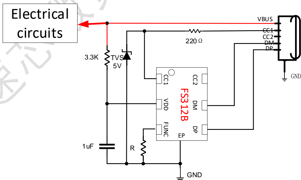
Figure 3. Application diagram
