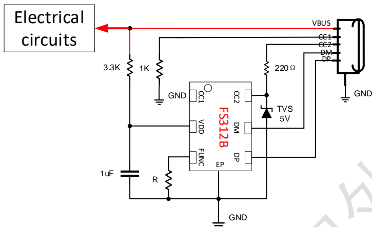
Figure 4. Application diagram
