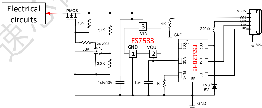
Figure 6. Application diagram
