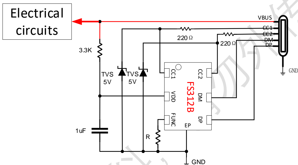
Figure 2. Application diagram
