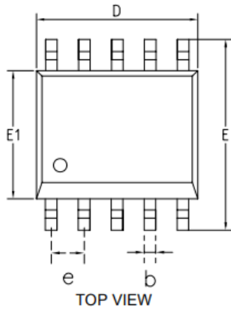
◆ ESSOP10 Package Outline Dimensions
